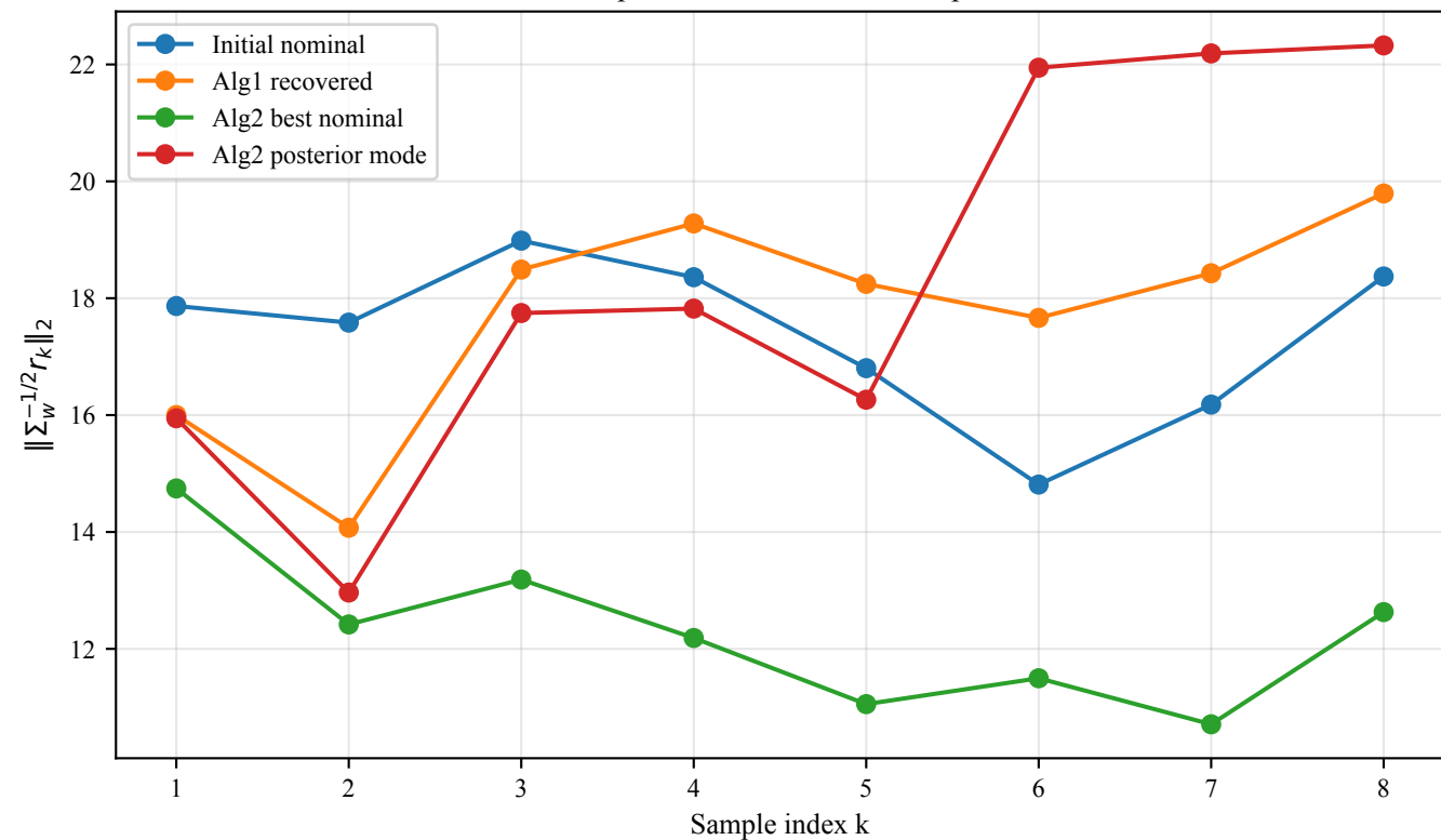
Per-sample whitened residual comparison
